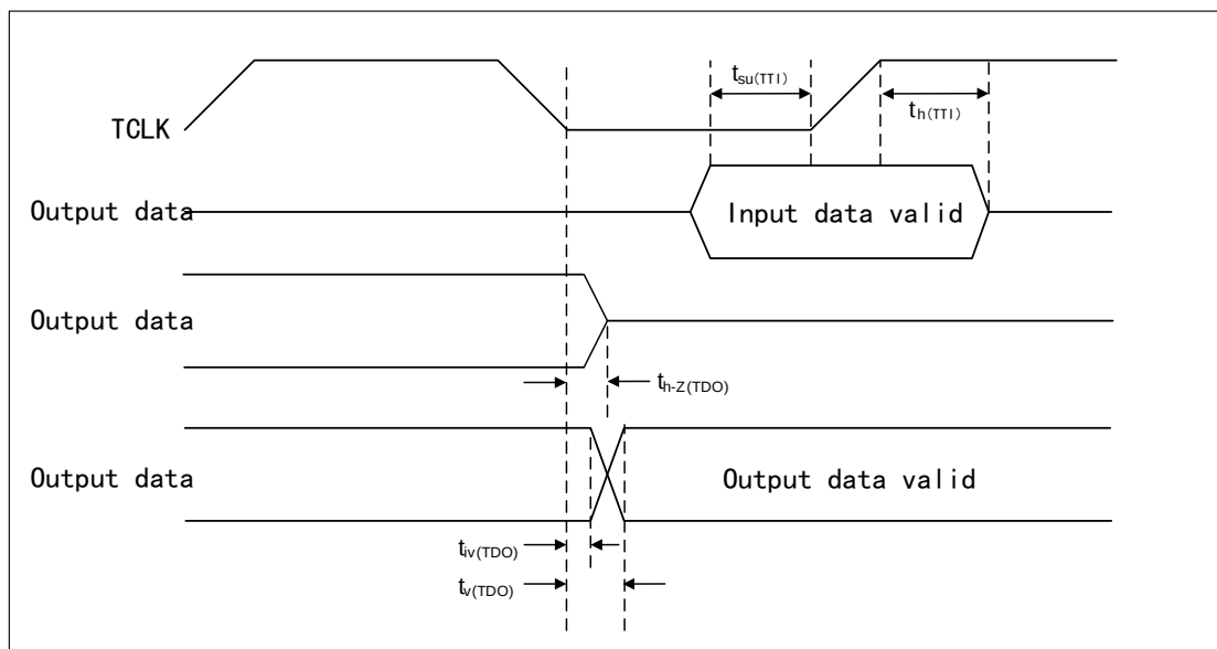
Figure 22 TDO Timing
