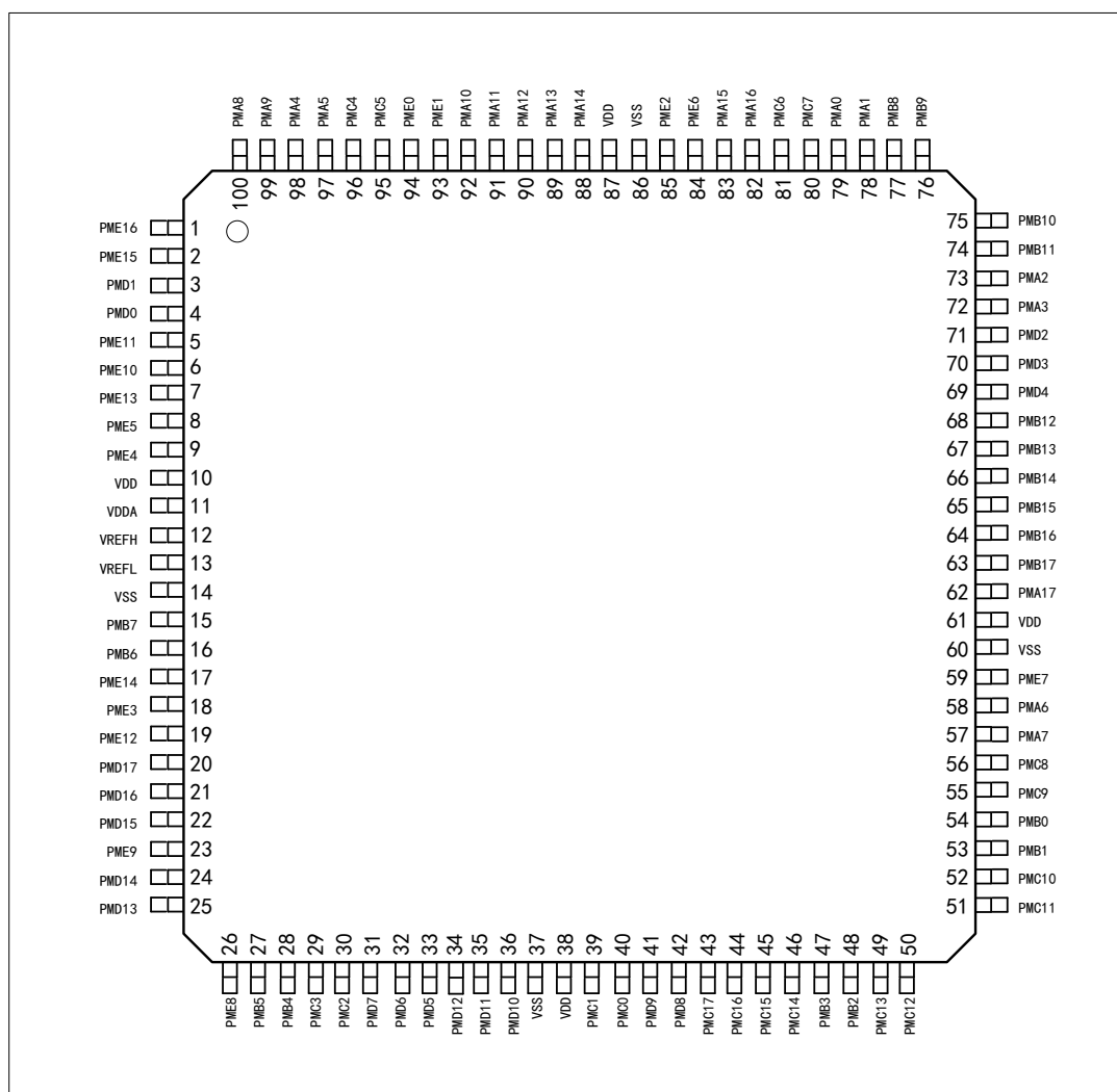
Figure 3 100-Pin LQFP Top View
