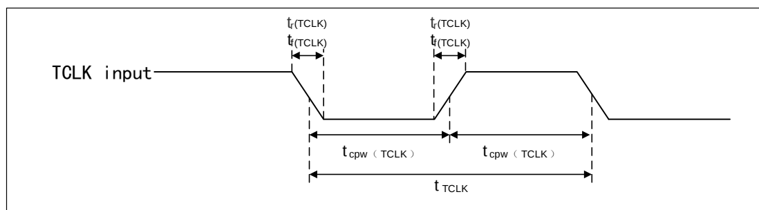
Figure 20 TCLK Input Timing
