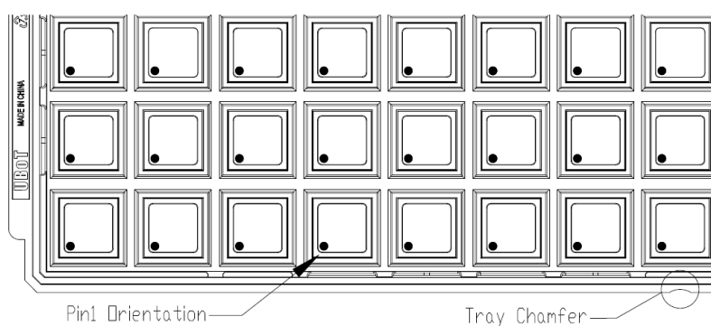
Figure 30 Tray Packaging Diagram
