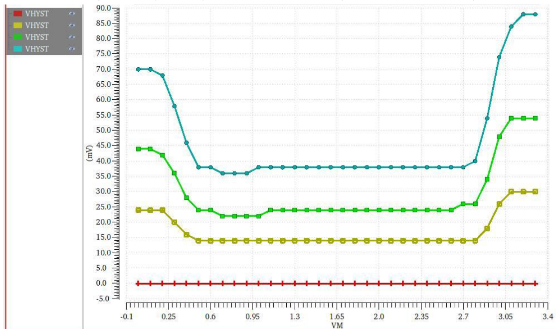
Figure 15 Typical hysteresis vs. Vin level ( V_{DDA}=3.3V, PMSEL=1 )
